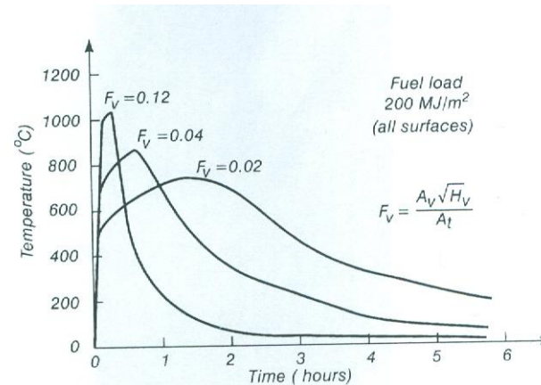
Figure 4.9 Time-temperature curves for varying ventilation and constant fuel load (MJ/m² total surface area)
