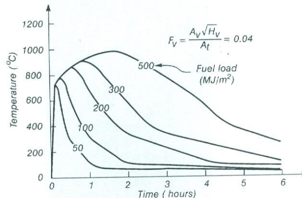
Figure 4.10 Time-temperature curves for varying fuel load (MJ/m² total surface area) and constant ventilation
